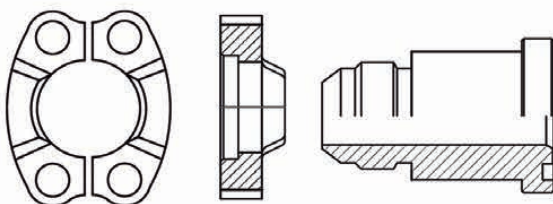
FLANGE ADAPTERS
